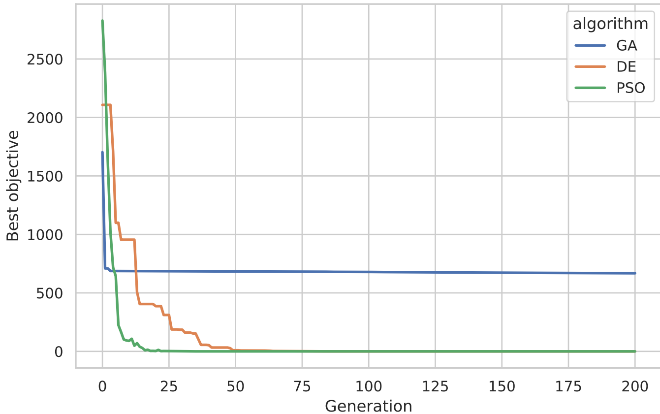
Algorithm Comparison
