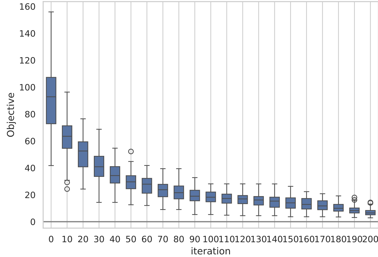
Fitness Distribution
