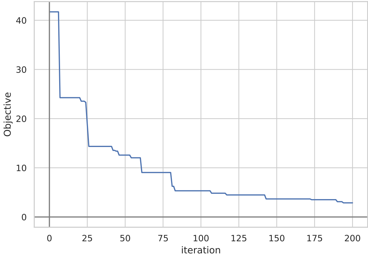
Best Objective
