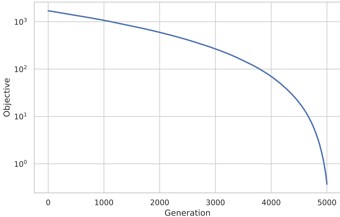
Convergence Plot
