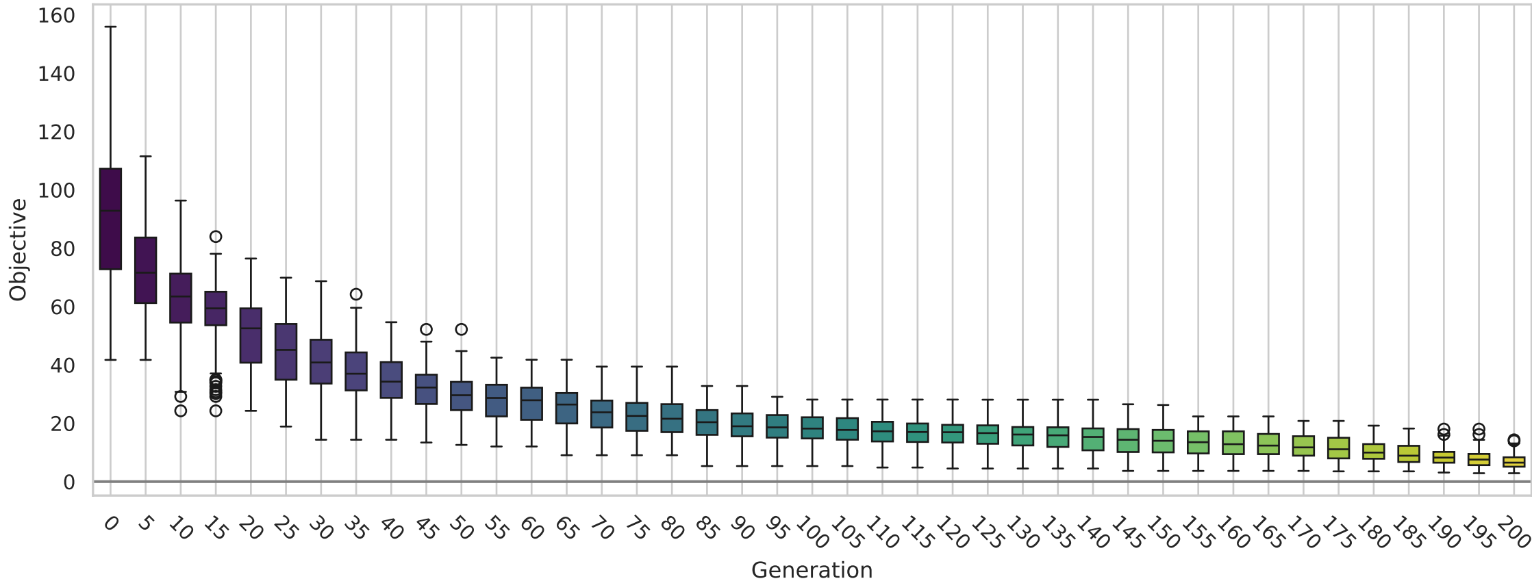
Fitness Distribution Every 5 Generations
